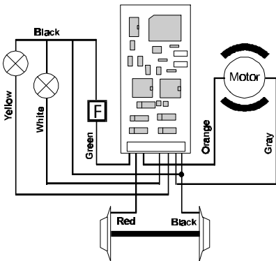
Figure 1: Wiring the LE102XF using track voltage common
