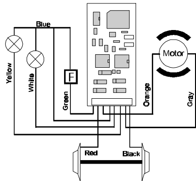
Figure 2: Wiring the LE102XF using a floating common.
