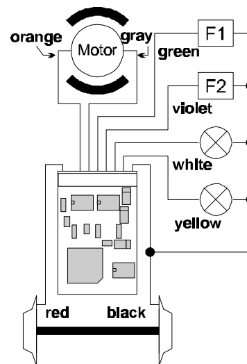
Figure 1: Wiring the LE110 using track voltage common
