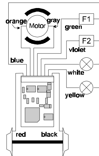
Figure 2: Wiring the LE110 using a floating common.
