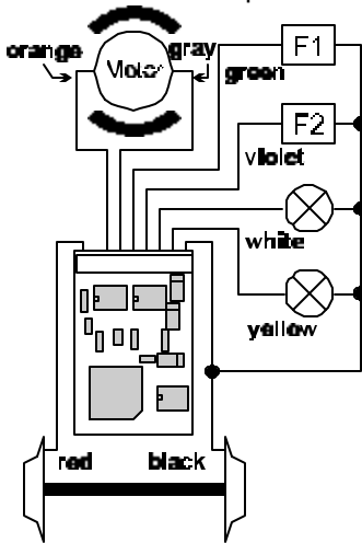
Figure 1: Wiring the LE113XF using track voltage common
