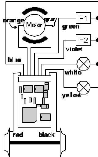
Figure 2: Wiring the LE113XF using a floating common.
