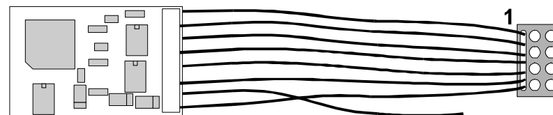
Figure 1: Wiring the LE135 Decoder
